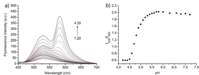
Fig. 23 (a) Fluorescence spectra of probe 18 (5 \mu M) in the B–R buffer/EtOH (9/1, v/v) solution at different pH values (7.20, 7.00, 6.80, 6.60, 6.30, 6.00, 5.80, 5.70, 5.60, 5.40, 5.30, 5.20, 5.10, 5.00, 4.90, 4.80, 4.70, 4.60, 4.50, 4.40, 4.30, and 4.20); and (b) the plot of the emission ratios of R at I_{529}/I_{580} versus pH values; \lambda_{\text{ex}} = 390 nm. Copyright 2015 Royal Society of Chemistry.
