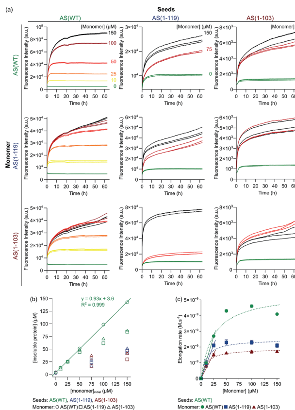
Fig. 2 Seeded aggregation of AS(WT), AS(1-119) and AS(1-103). (a) Change in the ThT fluorescence when seeds of AS(WT) (left), AS(1-119) (middle) or AS(1-103) (right) at a concentration of 5 \mu\text{M} (monomer equivalent) were incubated in the presence of increasing concentrations of monomeric AS(WT) (top), AS(1-119) (middle), AS(1-103) (bottom) at pH 6.5, 37 ^{\circ}\text{C} and under quiescent conditions. (b) Change in the concentration of insoluble proteins measured at the plateau phase of the aggregation reaction for different initial concentrations of monomers. (c) Change in the elongation rate when seeds of AS(WT) (5 \mu\text{M} in monomer equivalent) were incubated with increasing concentrations of AS(WT) (green), AS(1-119) (blue), AS(1-103) (red) monomers. The dotted lines show the fits of the data using the following equation, which describes the saturation behaviour of the elongation rate: 62 r(m_0) = \frac{r_{\text{max}}m_0}{m_{1/2} + m_0} . The linear fits to the low concentration data (solid lines) were used to obtain a robust measure of the elongation rate constant (see ESI† for more details†).
