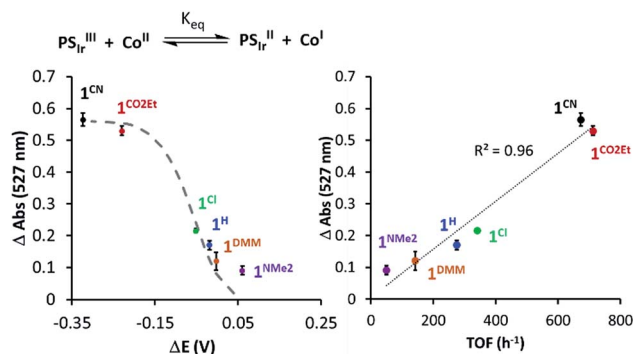
Fig. 7 (Left) The 527 nm absorbance decay upon addition of 1 R vs. ΔE 1/2 (PS Ir + /PS Ir ) - E 1/2 (Co II/I ). (Right) 527 nm absorbance of PS Ir decay upon addition of 1 R vs. TOF (h -1 ) (initial rate at 10% conversion of H 2 evolution). The dashed grey line refers to the theoretical values predicted from Nernst equation (see Section ESI 6.1†).
