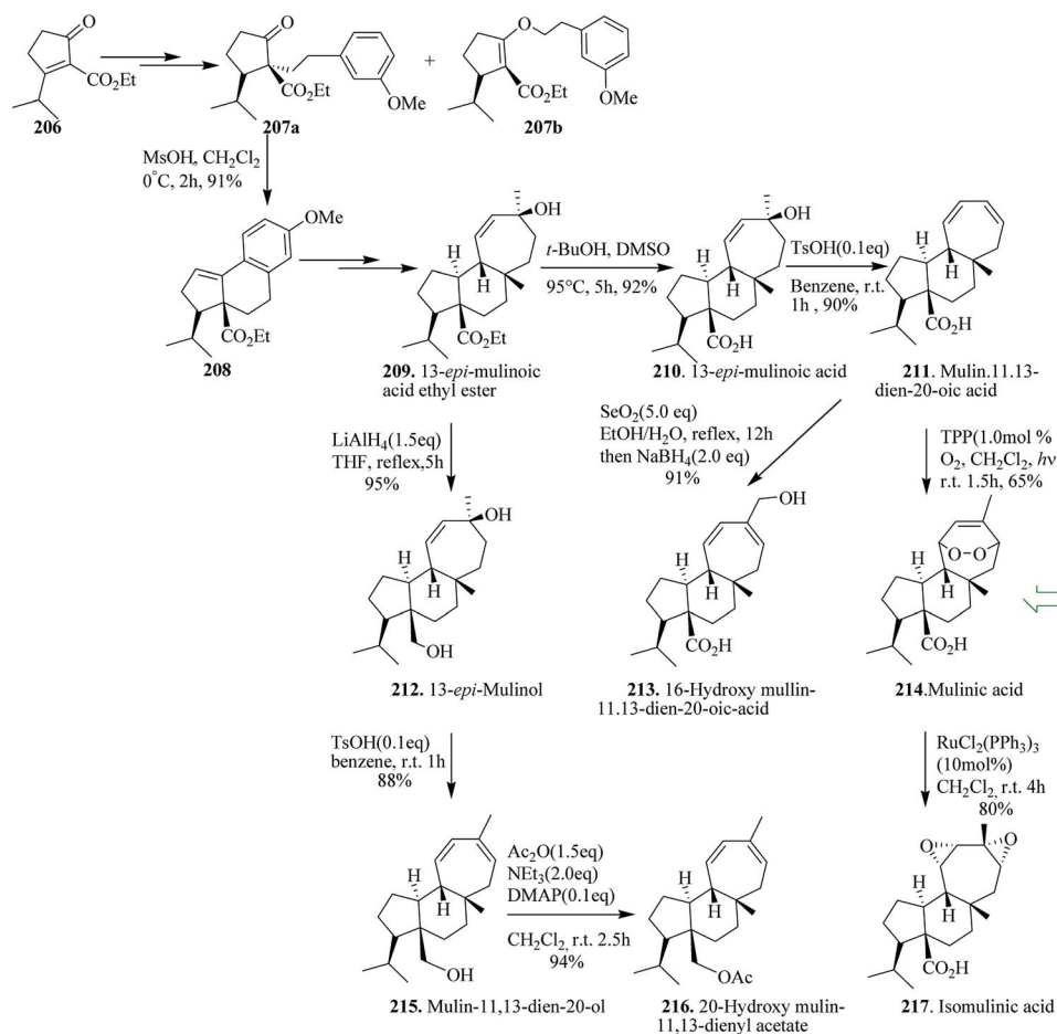
Scheme 45 Total synthesis of 13-epi-mulinolic acid ethyl ester 209 , 13-epi-mulinolic acid 210 , mulin-11,13-dien-20-oic acid 211 , 13-epi-mulinol 212 , 16-hydroxymulin-11,13-dien-20-oic acid 213 , mulinic acid 214 , mulin-11,13-dien-20-ol 215 , 20-hydroxymulin-11,13-dienyl acetate 216 and isomulinic acid 217 .
