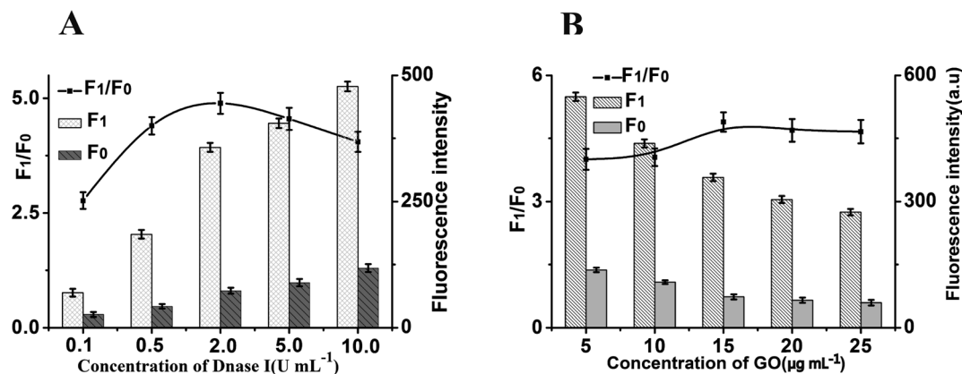
Fig. 3 (A) The effect of Dnase I concentration on the fluorescence response of this method. F_0 : control experiments; F_1 : with 5 ng mL -1 of MUC1, and the concentrations of probe is 40 nM. The black lines represent the F_1/F_0 at different conditions, while the F_1 and F_0 were the fluorescence intensities in the presence and absence of MUC1, respectively. Error bars: SD, n = 3 .
