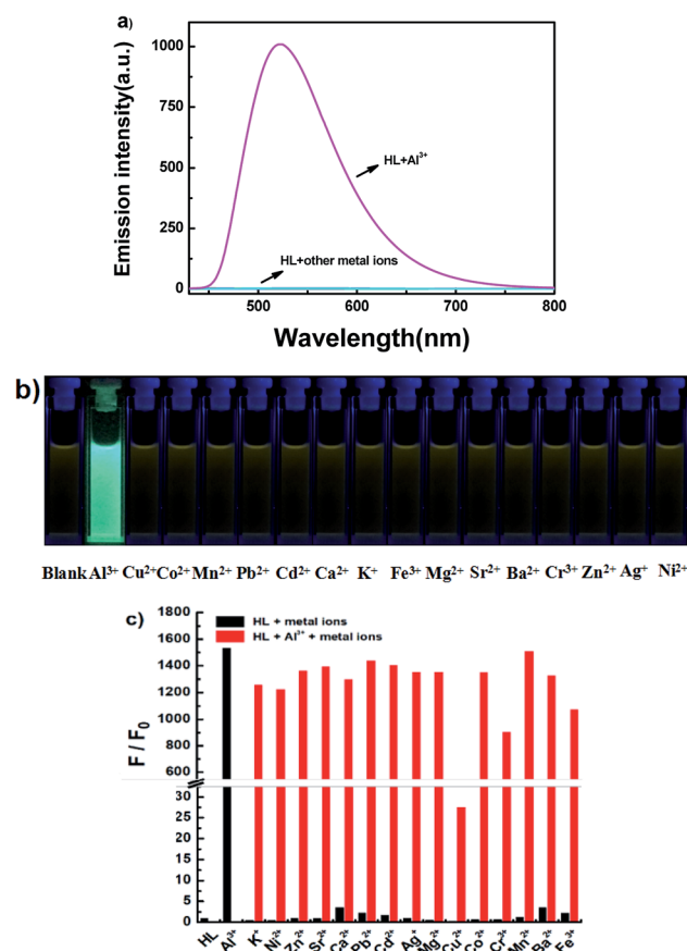
Fig. 5 (a) Fluorescence emission spectral changes of HL induced by various metal ions (5.0 equivalents) in acetonitrile ( 2.0 \times 10^{-5} \text{ mol L}^{-1} ) by excitation at 420 nm; (b) photos of fluorescence changes in acetonitrile; (c) the fluorescence intensity at 521 nm of HL upon addition of various metal ions (black bars: HL with metal ions; red bars: HL with other metal ions and \text{Al}^{3+} ) in acetonitrile.
