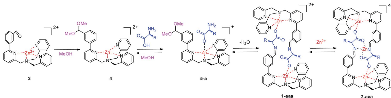
Scheme 1 Complex 3 dissolved in methanol give rise to the formation of acetal 4 within hours depending on the initial amount of water. Addition to this mixture of amino acid L-Phe leads to adduct 5-L-Phe which, in dry conditions, evolves to the dinuclear adduct complex 1-L-Phe or to complex 2-L-Phe in the presence of an excess of Zn(II) in solution. The counteranions are perchlorate.
