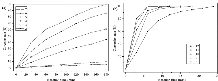
Fig. 8 Effects of pH on the catalytic oxidation. Reaction condition: methylene blue, 50 mL (10 mg L -1 ); catalyst, 4 mg; H 2 O 2 ; T = 25 °C.
