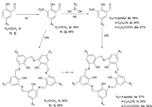
Scheme 2 Syntheses of campestarenes ( 1i–1m ): (x) \text{HNO}_3 , AcOH, 2 h; (xi) \text{Na}_2\text{CO}_3 , \text{Pd(PPh}_3)_4 , DMF/ \text{H}_2\text{O} , 105 °C, 6 h, then HCl; (xii) \text{Na}_2\text{S}_2\text{O}_4 , EtOH/ \text{H}_2\text{O} , reflux, 2 h.
