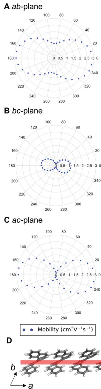
Fig. 8 Angular-dependent electron-mobility for structure 11 in the (a) ab -, (b) bc - and (c) ac -planes; (d) the adjacent translational homochiral chain (substructure type I ) with electron-mobility of 2.9 \text{ cm}^2 \text{V}^{-1} \text{s}^{-1} . The red arrow shows the highest electron-mobility direction for structure 11 .
