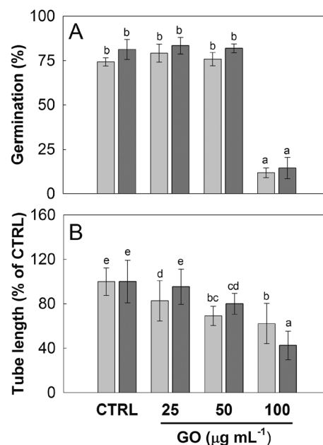
Fig. 4 Germination percentage (A) and pollen tube length (B) measured in Corylus avellana . Pollen germinated in BK suc without (CTRL) or with 25, 50 or 100 \mu\text{g GO mL}^{-1} after 3 h (grey bars) and 5.5 h (dark grey bars). Values are reported as means \pm 1 st. dev ( n = 150 for A; n \geq 50 for B). Statistically different groups are marked with different letters (two way ANOVA, Tukey's HSD post-hoc test).
