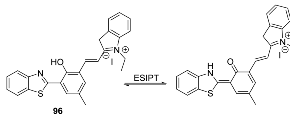
Scheme 84 A NIR-lysosomal targeting ESIPT + FRET probe 96 for the imaging of lysosomes in normal human lung fibroblast cells. Measurement conditions: H 2 O at various pH.
