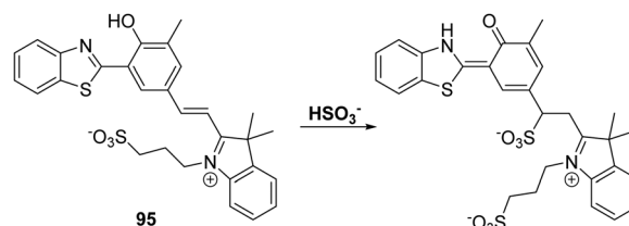
Scheme 83 A combined ICT + ESIPT fluorescent probe 95 for the detection of HSO 3 - . Measurement conditions: PBS/EtOH (6 : 4) – pH = 7.4.
