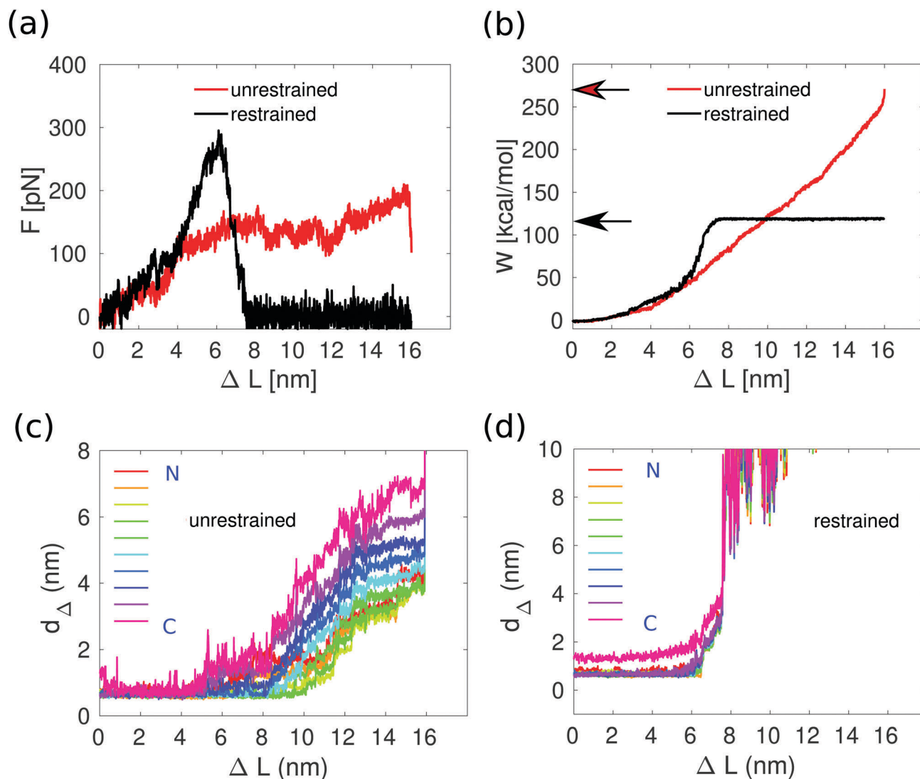
Fig. 4 Effect of helix stability on the deformation and rupture of the trimeric coiled coil at v = 10^{-2} nm ns ^{-1} . (a) Force–distance relationships with and without restraint potentials. The curves are obtained by averaging over four individual force traces for the unrestrained case (red) and over three such traces for the restrained case (black). (b) Toughness W as a function of extension \Delta L , calculated via eqn (1) from the forces in panel a. The arrows point to the toughness obtained when helix B separates from helices A and C. (c) Hydrophobic contacts as function of the extension: without restraint potentials. (d) Hydrophobic contacts as function of the extension: with restraint potentials. The hydrophobic contacts are quantified by the distances d_{\Delta} at each hydrophobic position a and d . d_{\Delta} is the average of distance of the sides of the triangle formed by the C_{\beta} atoms of the hydrophobic residues of each of the helices at the same position a or d . The colors indicate the position of these triangles along the CC bundle (up-to-down corresponds to the N-to-C terminus direction).
