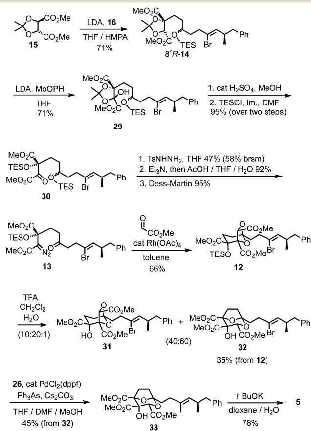
Scheme 6 Completion of the synthesis of (–)-6,7-dideoxysqualestatin H5 5 .
