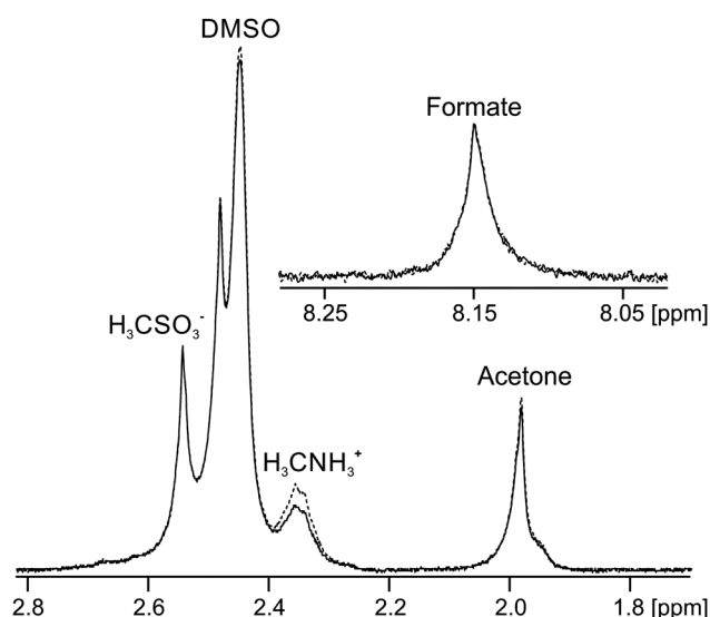
Fig. 7 ^1\text{H} NMR spectra of probe molecules in 3 /DMSO gel with (solid) and without (dashed) on resonance pre-saturation applied to the gel fibres. The downfield and upfield resonances of acetone and DMSO correspond to the totally protonated ( \text{H}_6 ) and partially deuterated ( \text{HD}_5 ) molecules respectively. The formate resonance is shown inset.
