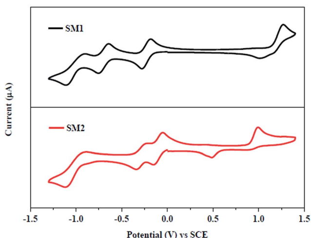
Fig. 2 Cyclic voltammogram of SM1 and SM2 at 0.01 M concentration in 0.1 M Bu 4 NPF 6 in chloroform recorded at a scan rate of 100 mV s -1 .
