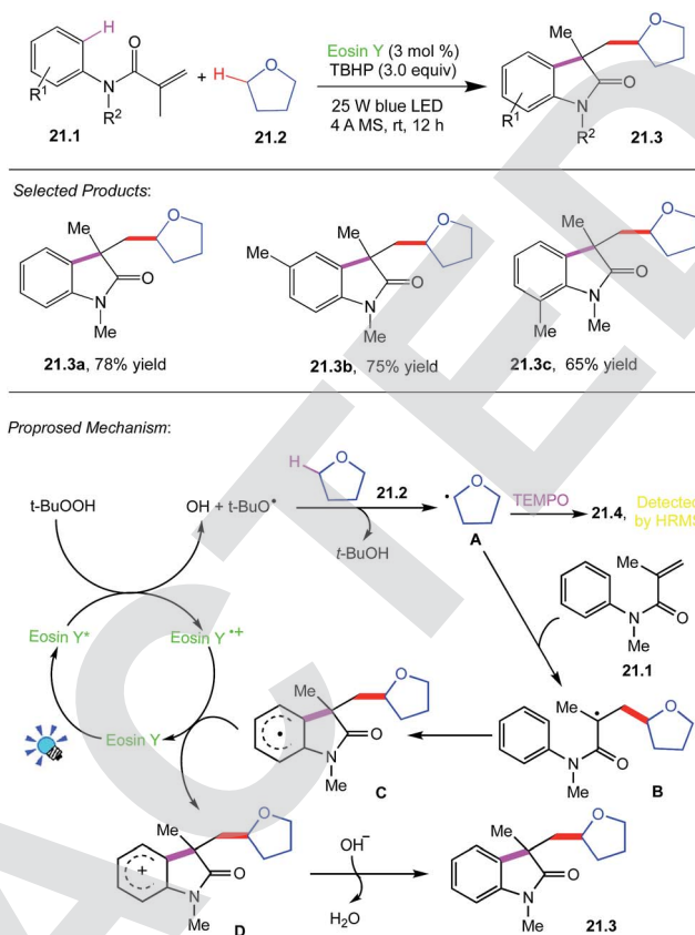
Scheme 21 Dual C–C bond formation via selective \text{C}(\text{sp}^3)\text{--H} bond cleavage.
