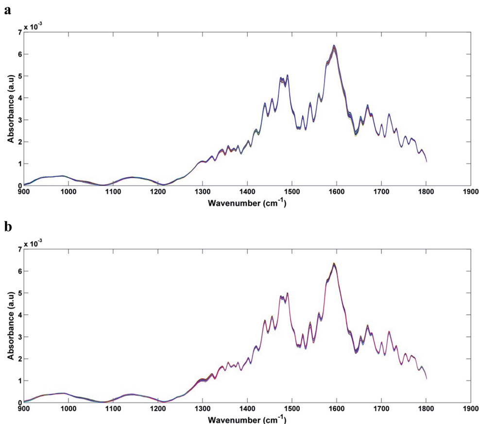
Fig. 2 Pre-processed spectra (cut between 900 and 1800 \text{cm}^{-1} , baseline correction and smoothing) of: (a) DENV-3 in serum ( 1 \times 10^3 , 1 \times 10^2 , 1 and 0.1 \text{PFU mL}^{-1} ); (b) DENV-3 in blood ( 1 \times 10^3 , 1 \times 10^2 , 10 and 0.1 \text{PFU mL}^{-1} ).
