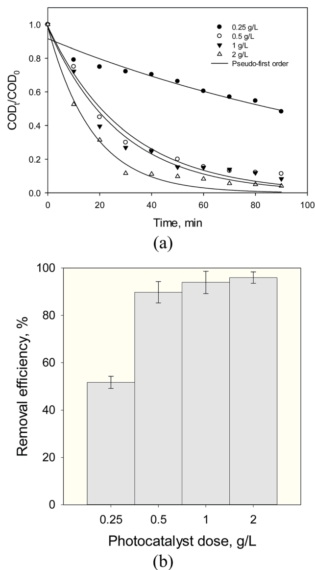
Fig. 10 (a) Kinetic curves, (b) removal efficiency of SMW with Fe_3O_4@TiO_2 (FT1) at different photocatalyst dose (pH = 3, 920\text{ mg L}^{-1} initial COD, 90 min reaction time and 30\text{ }^\circ\text{C} ).
