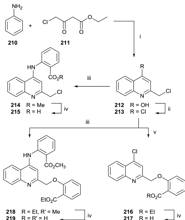
Scheme 37 Reagents and conditions: (i) PPA, 130^\circ C , 1 h. (ii) POCl_3 , 100^\circ C , 3 h. (iii) Methyl 2-aminobenzoate, C_2H_5OH , conc. HCl , 5 h. (iv) THF/MeOH , LiOH , 3 h. (v) Ethyl-2-hydroxybenzoate, K_2CO_3 , CH_3CN , 90^\circ C , 5 h.
