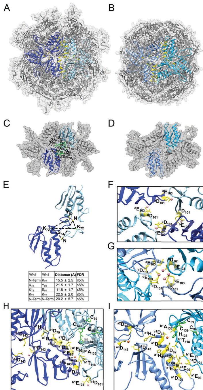
Fig. 8 Proposed iron binding sites in the [\text{Yfh1}]_{24}\text{-}[\text{Isu1}^{\text{LMW}}]_{24} complex. (A) Top view of two adjacent Yfh1 trimers at the 2-fold axis of the [\text{Yfh1}]_{24}\text{-}[\text{Isu1}^{\text{LMW}}]_{24} complex. Yfh1 trimers are shown as blue and light blue ribbons with proposed iron coordinating residues shown as yellow sticks. (B) Same as in (A) for the [\text{Yfh1}]_{24}\text{-}[\text{Isu1}^{\text{HMW}}]_{24} complex 16 with Yfh1 trimers shown as cornflower blue and deep sky blue ribbons. (C) PISA-identified interface between the two adjacent Yfh1 trimers at the 2-fold axis of the [\text{Yfh1}]_{24}\text{-}[\text{Isu1}^{\text{LMW}}]_{24} complex. Conserved residues within this interface predicted to form hydrogen bonds and hydrophobic interactions are shown as green sticks (see also Table 5 for additional details). The letters a and b denote the two adjacent Yfh1 trimers. (D) The interface shown in (C) is not present in the [\text{Yfh1}]_{24}\text{-}[\text{Isu1}^{\text{HMW}}]_{24} complex. (E) The interface shown in (C) fulfills the distance constraints set by the Yfh1–Yfh1 cross-links shown. The table underneath the structure provides the distances between each pair of cross-linked residues shown in the structure, and the False Discovery Rate (FDR) of the corresponding cross-linked peptides. See Table S1 (ESI†) for additional details. (F) Putative mineralization site at the 4-fold axis of the [\text{Yfh1}]_{24}\text{-}[\text{Isu1}^{\text{LMW}}]_{24} complex formed by four Yfh1 monomers that belong to four different Yfh1 trimers denoted by the letters a, b, c, and d. Iron atoms shown as pink spheres were modelled through alignment of the complex structure with the structure of cobalt-bound CyaY monomer (PDB: 2EFF). (G) As in (F) for the [\text{Yfh1}]_{24}\text{-}[\text{Isu1}^{\text{HMW}}]_{24} complex. 16 (H) Top view of the proposed path for iron delivery from Yfh1 to Isu1 in the [\text{Yfh1}]_{24}\text{-}[\text{Isu1}^{\text{LMW}}]_{24} complex. The path is formed by two adjacent Yfh1 trimers at the 2-fold axis as in (A). Three potential iron-binding sites were identified through alignment of the complex structure with the structures of iron-bound Yfh1 Y73A trimer (PDB: 2FQL, 4EC2) and cobalt-bound CyaY monomer (PDB: 2EFF). The letters a and b denote two adjacent Yfh1 trimers; the numbers 1, 2, and 3 denote different subunits of trimer a or trimer b. For Isu1, only the Fe–S cluster coordinating residues are shown as green sticks. (I) As in (H) for the [\text{Yfh1}]_{24}\text{-}[\text{Isu1}^{\text{HMW}}]_{24} complex. 16
