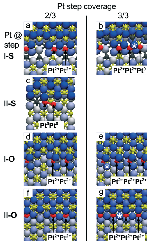
Fig. 9 Capacity of the CeO 2 (111) step edges to accommodate Pt 2+ ions obtained from DFT calculations. Calculated top views of Pt atoms bound to steps I-S (a and b), II-S (c) and I-O (d and e) for Pt step coverage 2/3 (a, c, d and f) and 1 (b, e and g). At step I-S, the limiting coverage of Pt 2+ is 2/3 (a), additional Pt attaches to the step edge as Pt 0 (b). At step II-S, the Pt 2+ coverage is 0. Pt atoms attach as weakly ionized Pt 4+ and readily form metallic dimers (c) and clusters. On both steps I-O and II-O, excess oxygen can stabilize ionic Pt 2+ at step edges as single ions appearing isolated or in groups up to 100% step coverage (d–g). Reproduced with permission from ref. 22, Copyright 2016, Nature Publishing Group.
