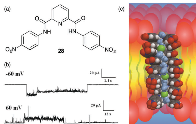
Fig. 4 Transmembrane chloride transport by (a) 4,4'-dinitrophenylamine 28 appears to occur via a channel mechanism: (b) the current observed at applied voltages of -60 mV and +60 mV upon addition of transporter 28 to a planar bilayer (c) DFT-calculated molecular model showing a stack of 10 molecules of 28 , 3 chloride anions and 16 water molecules. The distance between the most distal monomers in the stack is approximately 3.4 Å. Reproduced from ref. 15. Copyright 2010, Royal Society of Chemistry.
