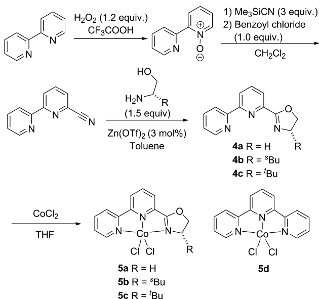
Scheme 2 Synthesis of bipyridiyl-oxazoline cobalt complexes 5a–5c and terpyridine cobalt complex 5d .
