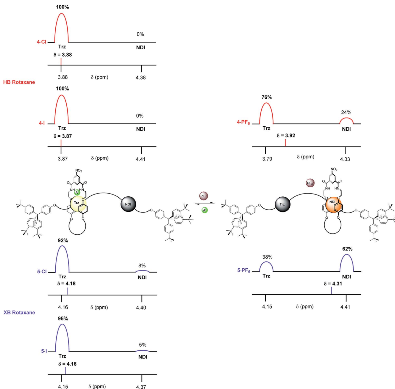
Fig. 7 The estimated percentage occupancies (based upon \text{H}_t protons) of the HB and XB rotaxanes 4·A and 5·A as chloride, iodide and \text{PF}_6^- salts as determined by ^1\text{H} NMR spectroscopy in \text{CDCl}_3 solution. \text{A}^- = \text{Cl}^- or \text{I}^- and Trz = triazolium.
