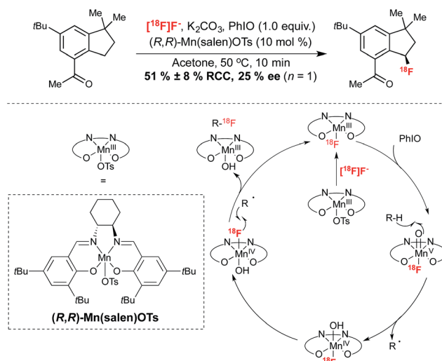
Scheme 4 Enantioselective benzylic ^{18}\text{F} -fluorination with [ ^{18}\text{F} ]fluoride through C–H functionalization.
