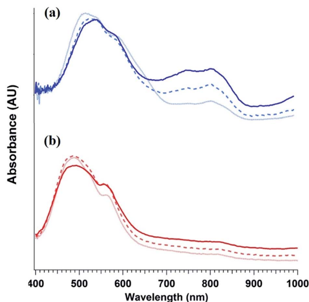
Fig. 4 Evolution PDI thin film optical absorption spectra with anneal time: 0 min (light dotted line), 20 min (dashed line), and 1 h (dark solid line) for (a) PDI-OH and (b) PDI-NMe 2 .
