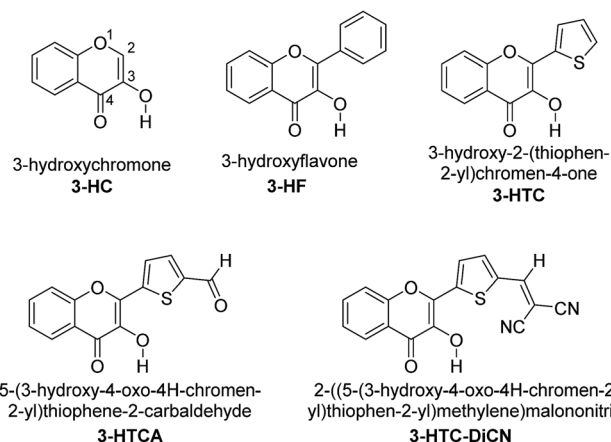
Chart 1 The chemical structures of 3-HC, 3-HF, 3-HTC, 3-HTCA and 3-HTC-DiCN.
