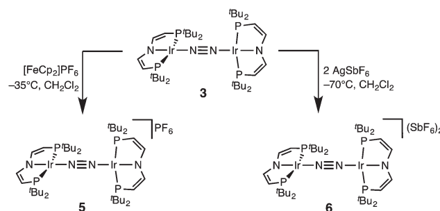
Scheme 2 Chemical oxidation of iridium(I)/iridium(I) \text{N}_2 -complex 3 .
