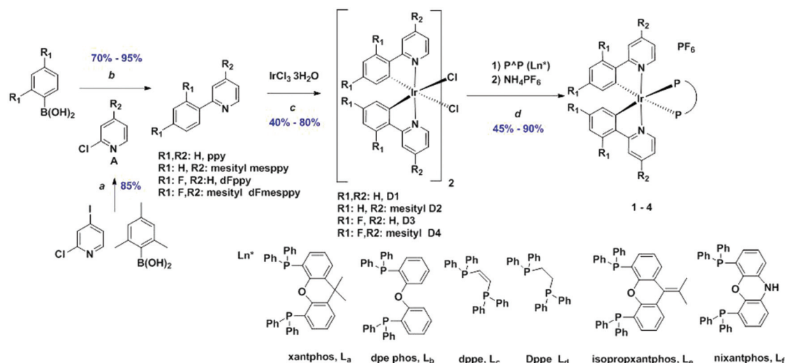
Scheme 1 Synthesis of C N ligands and [Ir(C N ) 2 (P AP )]PF 6 complexes 1–4 . Reagents and conditions. a 2.0 equiv. K 2 CO 3 , 5 mol% Pd(PPh 3 ) 4 , N 2 , 1,4-dioxane/H 2 O (4 : 1 v/v), 105 °C, 56 h; b 2.0 equiv. K 2 CO 3 , 5 mol% Pd(PPh 3 ) 4 , N 2 , 1,2-dimethoxyethane/H 2 O (4 : 1 v/v), 130 °C, 19 h; c 2-EtOC 2 H 4 OH/H 2 O (4 : 1 v/v), 110 °C, N 2 , 19 h. d i. CH 2 Cl 2 /MeOH (2 : 1 v/v), 55 °C, 19 h, N 2 ; ii. Excess solid NH 4 PF 6 .
