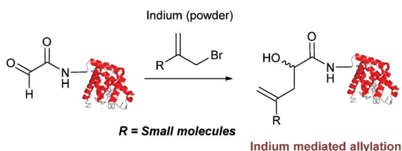
Scheme 13 Outline of an indium mediated allylation of glyoxyl-myoglobin.
