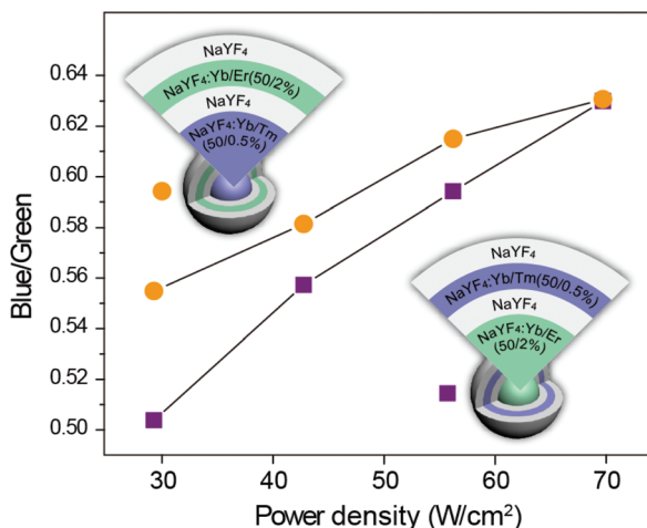
Fig. 7 Power dependent blue-to-green upconversion emission intensity ratio of NaYF 4 :Yb/Tm@NaYF 4 :Yb/Er@NaYF 4 and NaYF 4 :Yb/Er@NaYF 4 :Yb/Tm@NaYF 4 UCNP upon 975 nm laser irradiation.
