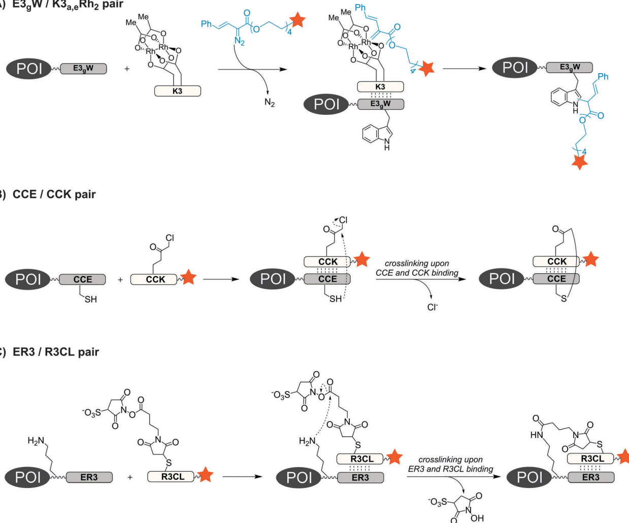
Fig. 7 Protein labelling via formation of coiled-coils. (A) Covalent labelling via rhodium-catalyst containing K3 peptide and diazo probe, (B) proximity induced covalent cross-linking between electrophilic \alpha -chloroacetyl group and thiol side chain and (C) proximity induced amine-reactive crosslinking.
