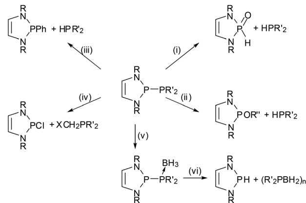
Scheme 6 Selected metathesis reactions of phosphino-DAPs. Reagents and conditions: (i) H 2 O, r.t. (R = Dipp, PR' 2 = PCO); (ii) R''OH, r.t. (R = tBu, Mes, R' = Ph, R'' = alkyl); (iii) R'OH, r.t. (R = Dipp, PR' 2 = PCO); (iv) ClCH 2 X, r.t. (R = tBu, Mes; R' = Ph, X = Cl); (v) BH 3 -thf, –10 °C (R = tBu, R' = Ph), (vi) r.t. (R = tBu, R' = Ph).
