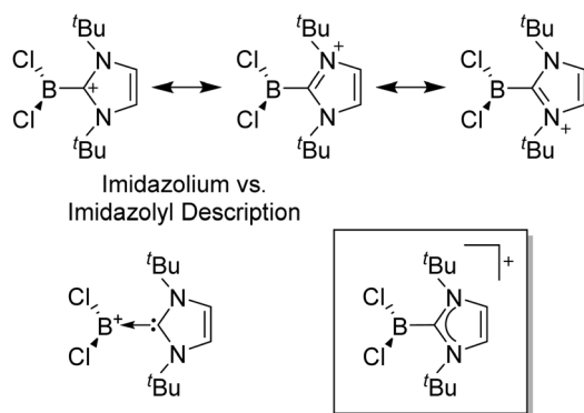
Fig. 3 Possible descriptions of NHC-containing structures exemplified for the simple [\text{Cl}_2\text{B}-\text{tBu}]^+ cation.
