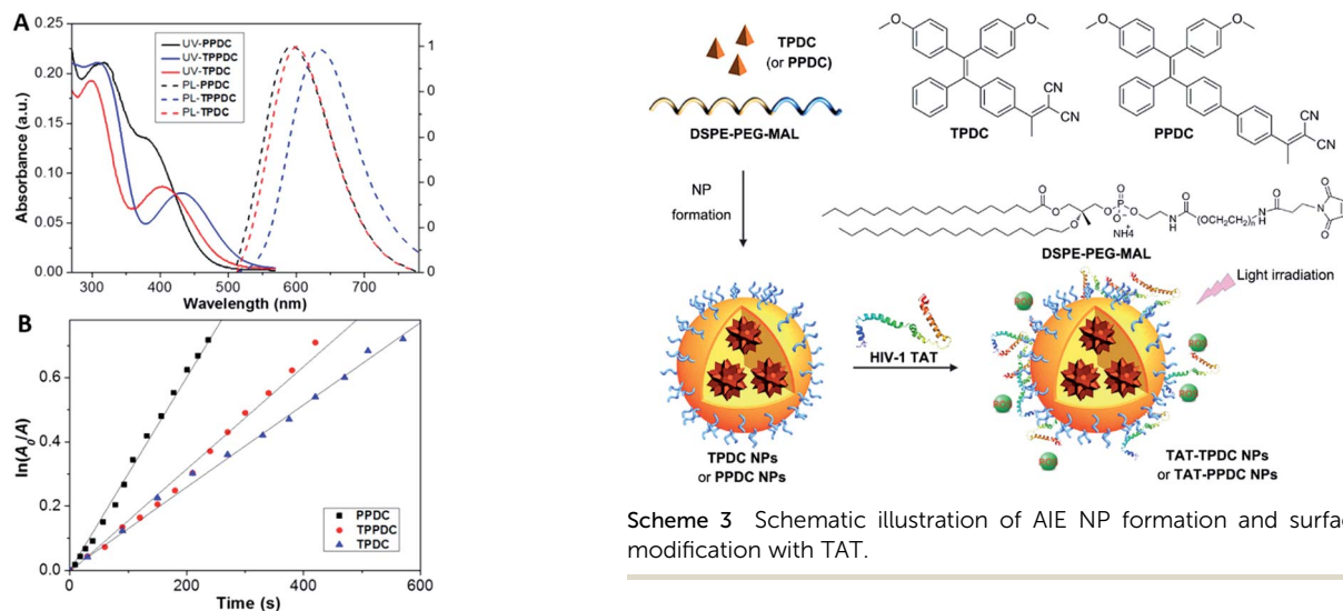
Fig. 3 (A) UV-vis absorption (solid lines) and normalized photoluminescence (PL) spectra (dashed lines) of 10 \mu\text{M} each of PPDC, TPDC and TPPDC in DMSO/water (v/v = 1/99). (B) The decomposition rates of ABDA by PPDC, TPDC and TPPDC; A_0 and A are the absorbance of ABDA in the presence of the AIEgen PSs at 378 nm before and after irradiation, respectively.
