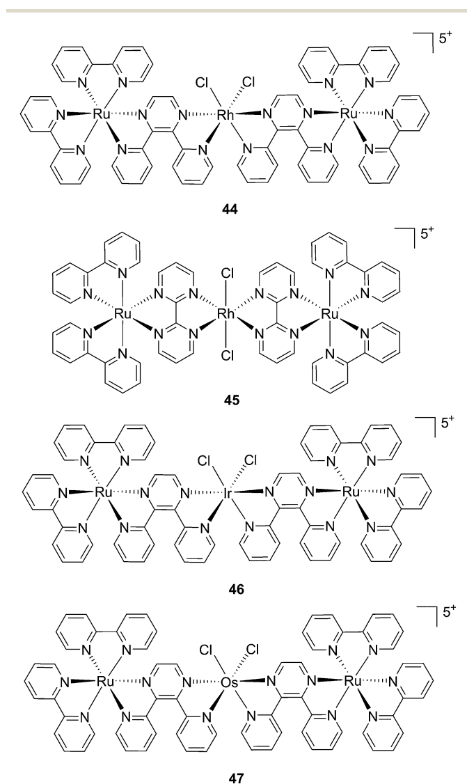
Fig. 31 Structures of the mixed-metal supramolecular complexes; ( 44 ) [\{(\text{bipy})_2\text{Ru}(\text{dpp})\}_2\text{RhCl}_2]^{5+} , ( 45 ) [\{(\text{bipy})_2\text{Ru}(\text{bpm})\}_2\text{RhCl}_2]^{5+} , ( 46 ) [\{(\text{bipy})_2\text{Ru}(\text{dpp})\}_2\text{IrCl}_2]^{5+} , and ( 47 ) [\{(\text{bipy})_2\text{Ru}(\text{dpp})\}_2\text{OsCl}_2]^{5+} . 97,99
