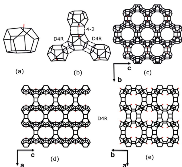
Fig. 3 Construction of the framework structure of ITQ-54. (a) The new [4 3 5 6 6 1 ] CBU. (b) Connectivity of the new CBU to the other three CBUs via D4R, D4R and 4–2 units, respectively, to form (c) a layer in the bc -plane with 12-ring pores. (d and e) The 12-ring layers connect to each other via D4Rs to form a 3D framework. 14-ring channels are created along the b -axis (d) and 20-ring channels are created along the c -axis (e). Only T–T connections and the terminal O atoms (in red) are shown.
