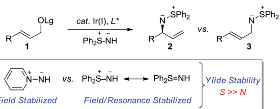
Scheme 1 Enantiospecific and enantioselective metal-catalyzed allylic amination reactions with aza-ylides.
