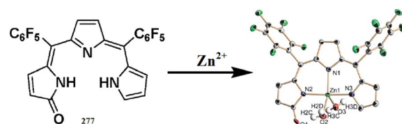
Fig. 241 Chemical structure of receptor 277 and the ORTEP view of the receptor-zinc complex.
