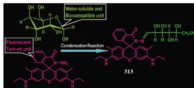
Fig. 275 Chemical structure of ligand 313 .
