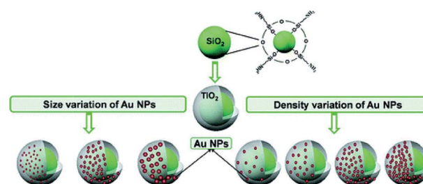
Fig. 5 Schematic illustration of the preparation protocol of core-shell \text{SiO}_2/\text{TiO}_2 nanostructures (silica bead coated with a thin layer \text{TiO}_2 of 15–20 nm in thickness) and the decoration of the \text{SiO}_2/\text{TiO}_2 surface with Au NPs. Figure reprinted with permission from ref. 70.
