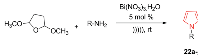
Scheme 4 Synthesis of N -substituted pyrrole derivatives by an eco-friendly route using ultrasound-assisted bismuth nitrate-catalyzed reaction.
