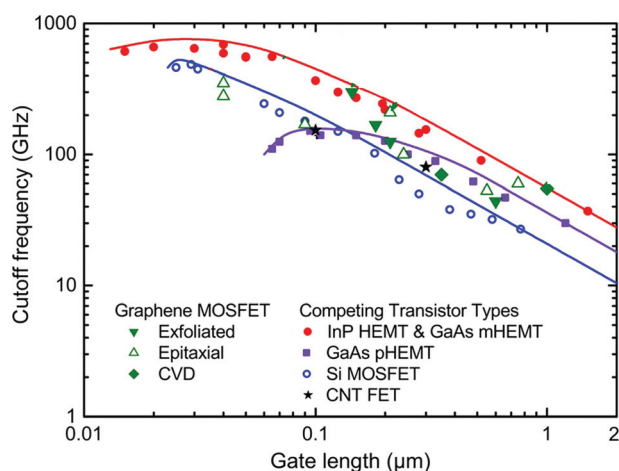
Fig. 62 Cut-off frequency versus gate length for GFETs, nanotube FETs and three types of RF-FETs [Adapted from ref. 1193]. pHEMT = pseudo-morphic HEMT, mHEMT = metamorphic HEMT. HEMTs are made of heterojunctions, i.e. , junctions of different materials. 1194,1195 The most common example are GaAs HEMTs in which there are junctions between \text{Al}_x\text{Ga}_{(1-x)}\text{As} and GaAs. Different materials have different lattice constants, hence crystal defects are expected in HEMTs. In pHEMTs this is avoided by using a very thin layer of one material 1196 so that accumulated energy in this layer is not enough to relax the layer and introduce defects (energy is low because the layer is very thin). 1196 In mHEMTs a graded buffer layer is used in between the layers to accommodate both lattice constants 1196 and eliminate the defects. E.g. , to grow \text{Al}_{0.3}\text{Ga}_{0.7}\text{As} on GaAs, an \text{Al}_x\text{Ga}_{(1-x)}\text{As} layer is grown first in which x = 0 at the beginning (GaAs) and then x is gradually increased to 0.3 ( \text{Al}_{0.3}\text{Ga}_{0.7}\text{As} ). 1196
