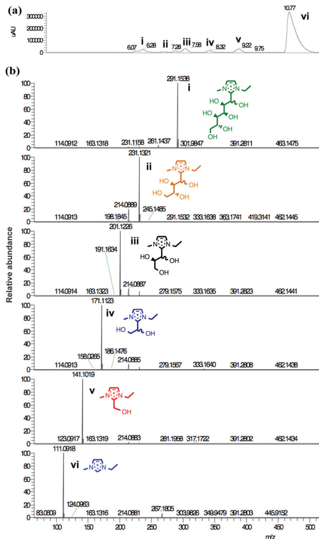
Fig. 4 LCMS investigation of adduct species formed from [C 2 C 1 im]-[OAc], 1a + 10 wt% D-(+)-glucose, 12 , heated to 120 °C for one hour (t 1 ): (a) survey of peaks i–vi; (b) ESI mass spectra of peaks i–vi.
