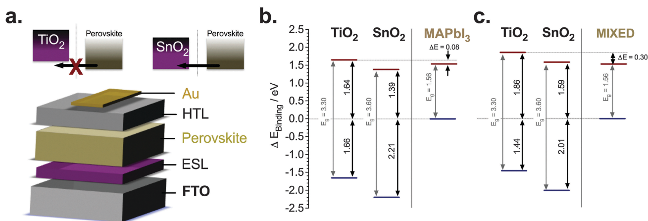
Fig. 1 Energy level diagrams and electron injection characteristics of \text{SnO}_2 and \text{TiO}_2 -based planar PSCs. (a) Schematic conduction band diagram of the perovskite films and the electron selective layers, \text{TiO}_2 and \text{SnO}_2 for (b) \text{MAPbI}_3 and (c) (\text{FAPbI}_3)_{0.85}(\text{MAPbBr}_3)_{0.15} , labeled as 'mixed'.
