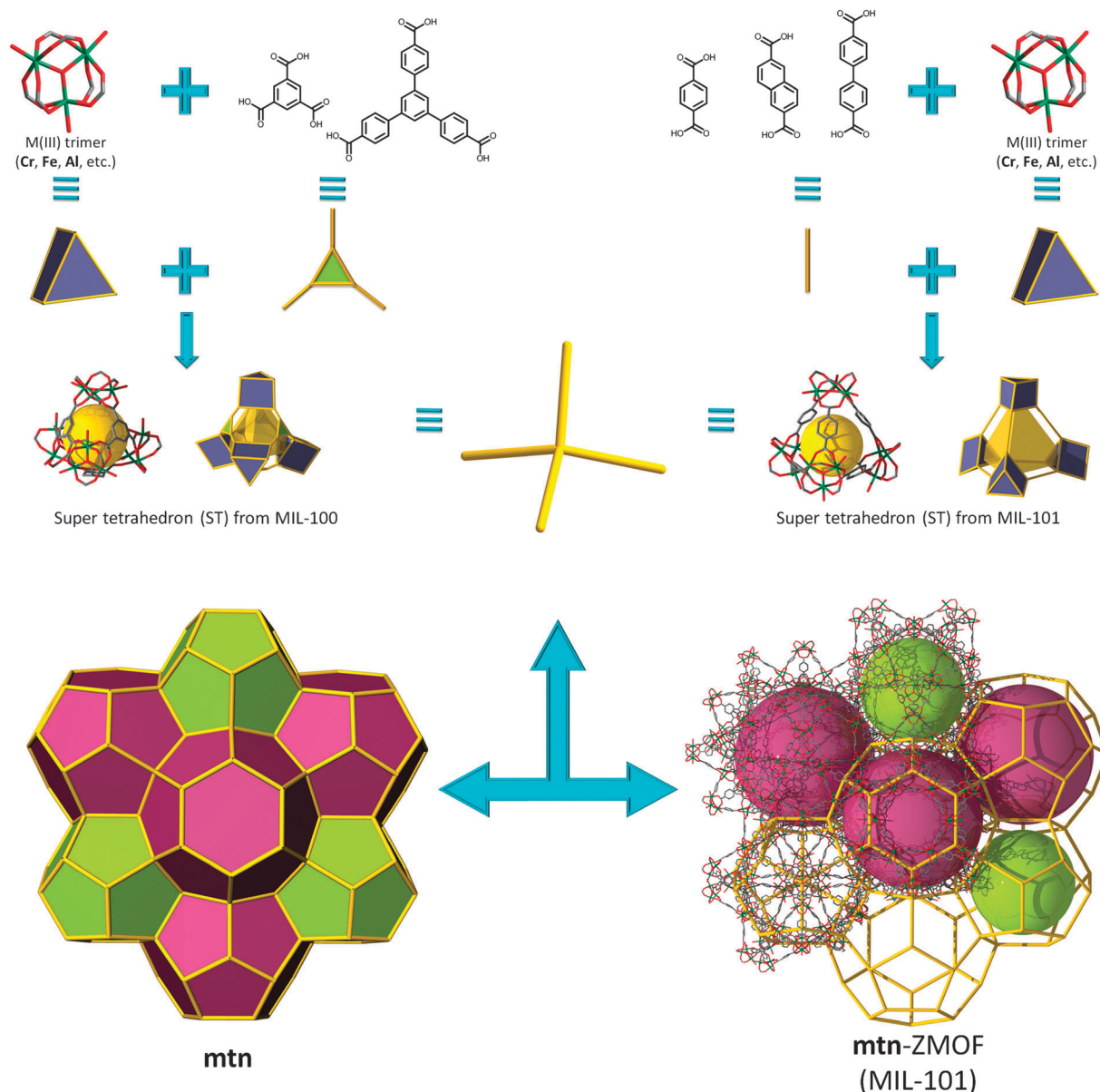
Fig. 18 Supertetrahedron (ST) building units based on M^{\text{III}} trimers and triangular (MIL-100's, left) or linear (MIL-101's, right) leading to the assembly of gigantic mtn -ZMOFs.
