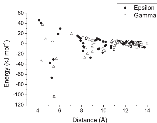
Fig. 10 Plot of contact energies (kJ mol -1 ) against centroid-centroid distance (Å) in \epsilon (filled circles) and \gamma -glycine (open triangles). Energies were calculated using the PIXEL method.
