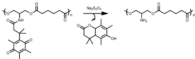
Scheme 10 TMBO shed from the polymer backbone upon reaction with sodium dithionite. 82
