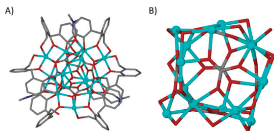
Fig. 2 (A) Part of the asymmetric unit in the structure of 1 . (B) Polymetallic skeleton in 1 showing the arrangement of the \mu_6-CO_3^{2-} anions.
