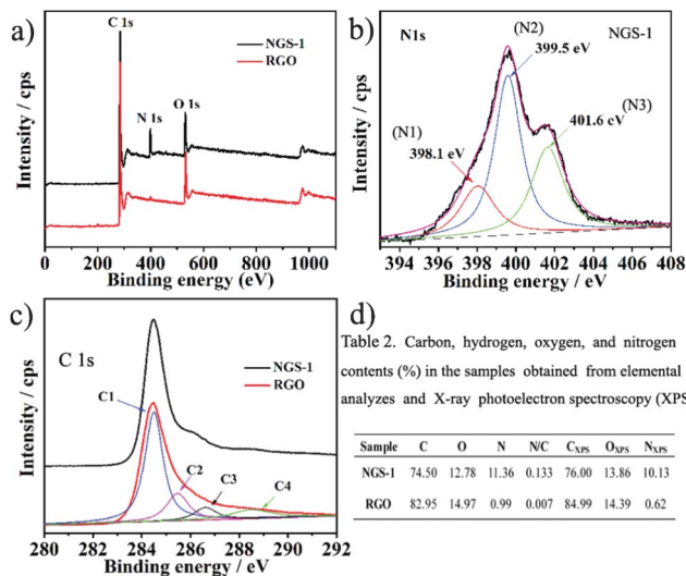
Fig. 3 a–c) XPS wide spectra, N1s spectra and C1s spectra of the synthesized NGS-1 and RGO samples, respectively; d) Elemental content and chemical composition in NGS-1 and RGO samples tested by elemental analysis and XPS.
